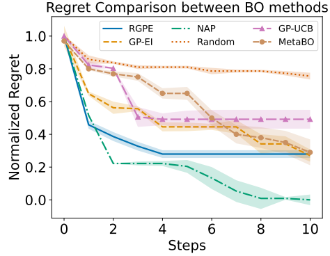
Figure 4: Comparison between classic BO methods and Meta-BO methods in ICF. NAP is able to achieve optimal performance in few-samples. The shaded areas represent a \pm 1 standard error. Regrets are normalized.
