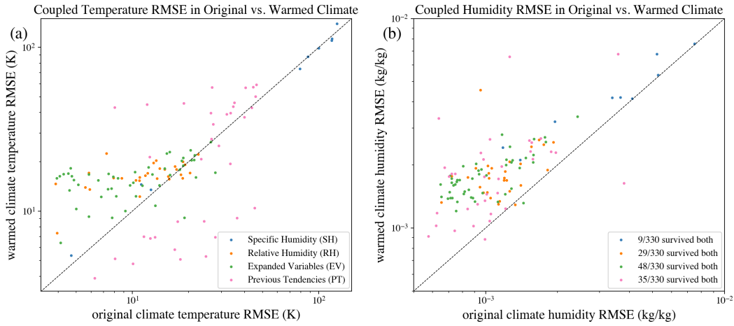
Figure 3: Scatterplots of coupled error for hybrid physics-ML simulations that did not prematurely terminate in either climate. Dashed line is a 1-to-1 line that intersects the origin.
