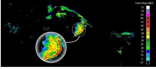
Figure 2. Radar image of the Continental United States with a bow echo, May 24, 2008, 10:20 GMT. We magnify the part that bow echo happened ( i.e. red regions).
