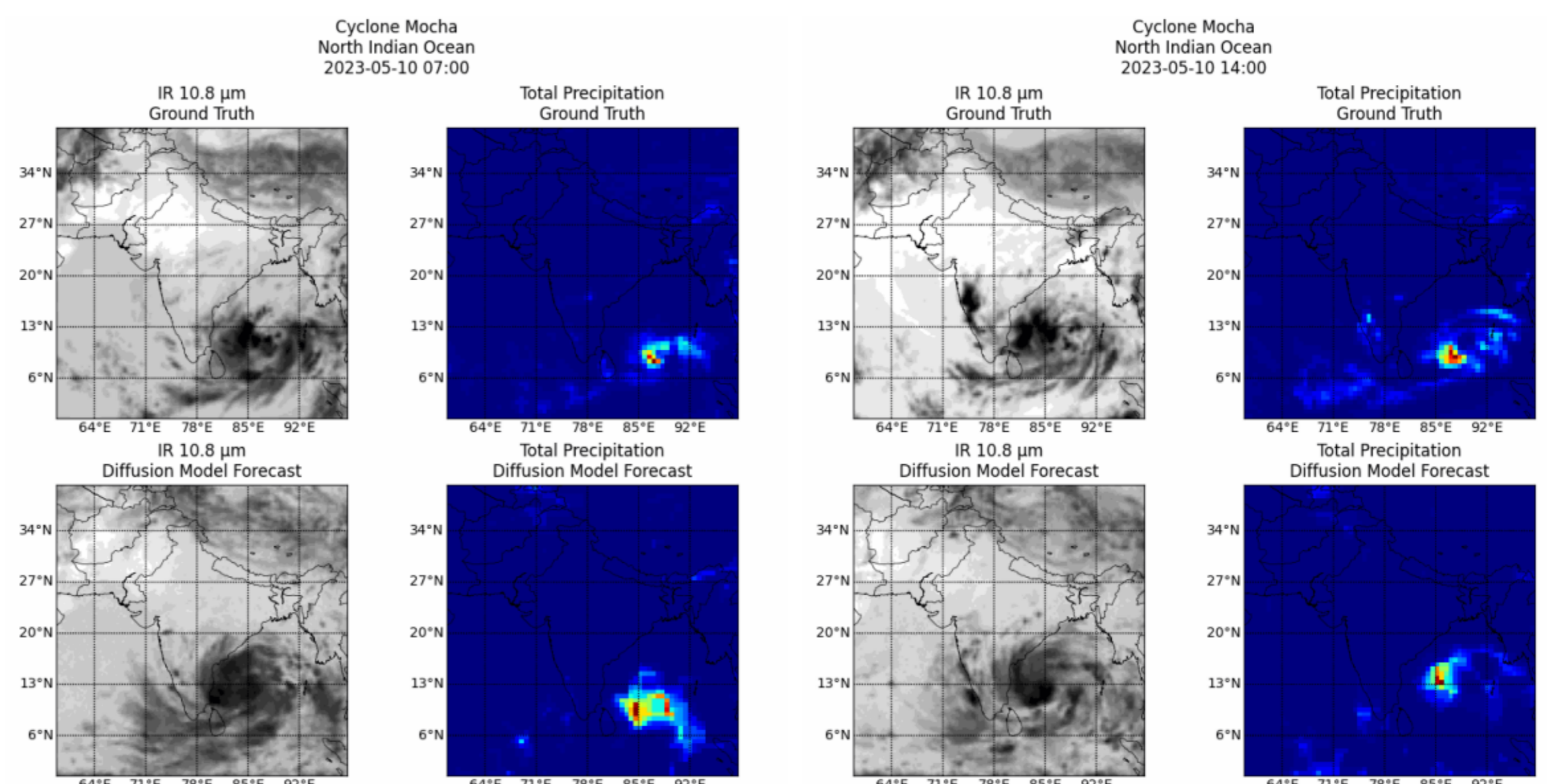
Figure 2: Forecast at 31h (left) and 38h (right) of Cyclone Mocha over the North Indian Ocean on 10th May 2023. The upper rows resemble the ground truth IR 10.8 \mu\text{m} satellite image and total precipitation while the lower rows show the forecast generated at that particular timestep.
