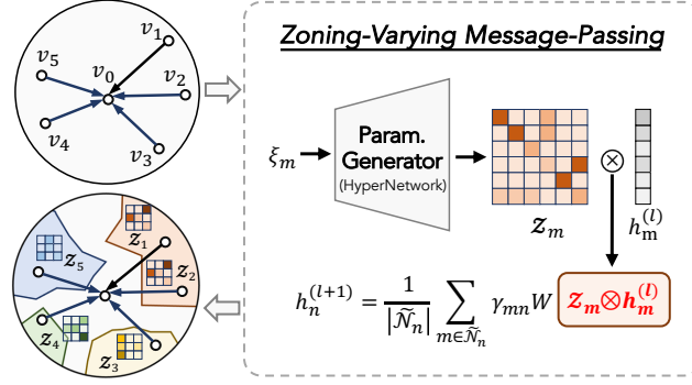
Figure 5: Framework of zoning-varying message-passing.
