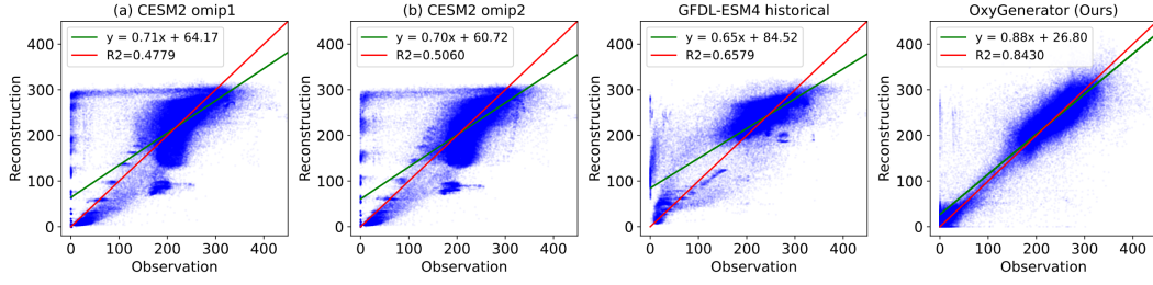
Figure 7: Performance Comparison of deoxygenation reconstruction of different numerical simulation methods and OXYGENERATOR in the Black Sea.
