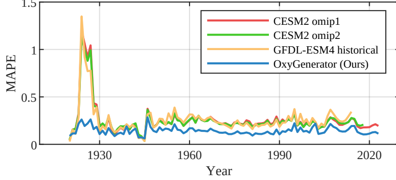
Figure 6: Performance Comparison of MAPE over time.
