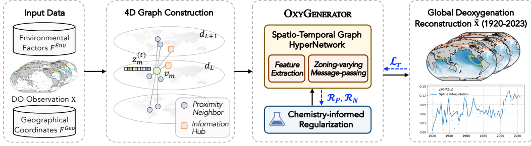
Figure 1: Framework of breathless ocean reconstruction via our proposed OXYGENERATOR.
