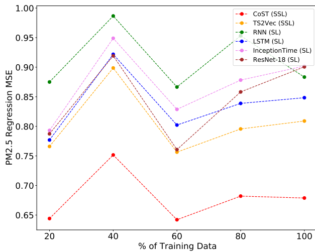
Figure 2: MSE on PM2.5 regression varying the amount of training data
